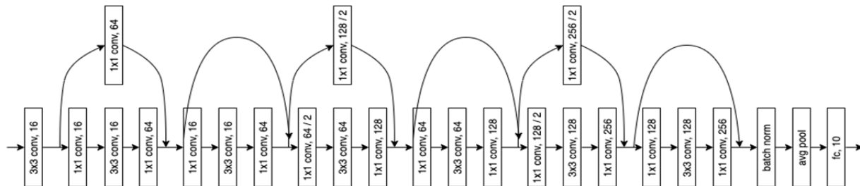
Fig. 3. The ResNet architecture with 22 convolutional layers used in experiments. Batch normalization and activations are omitted for simplicity
